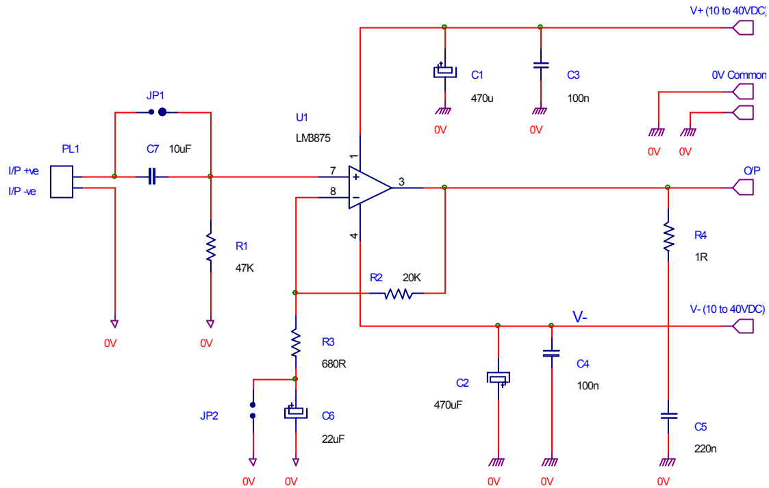
AMP50 Monoblock power amplifier
